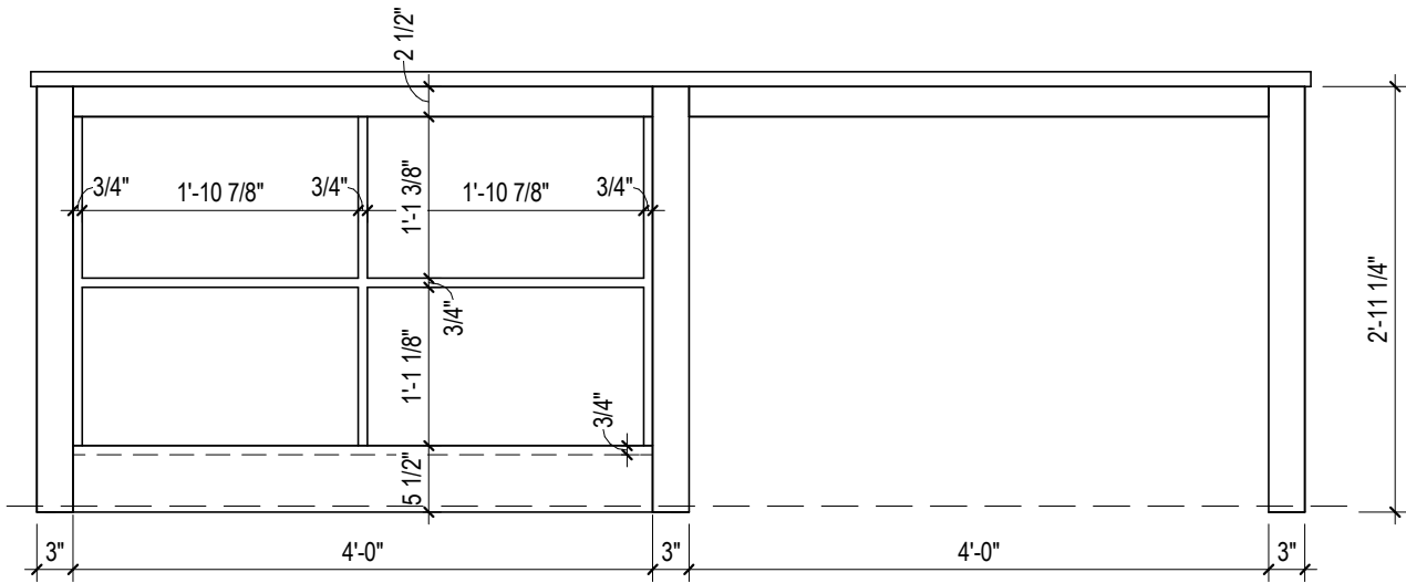
KITCHEN ISLAND - SHELF ELEVATION
