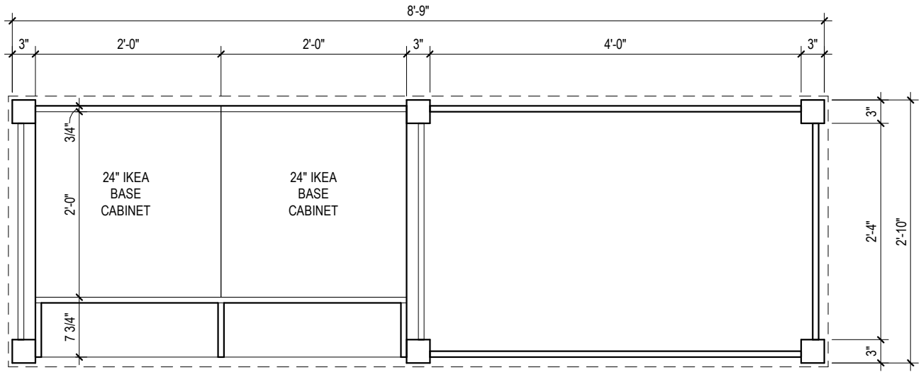
KITCHEN ISLAND - PLAN
